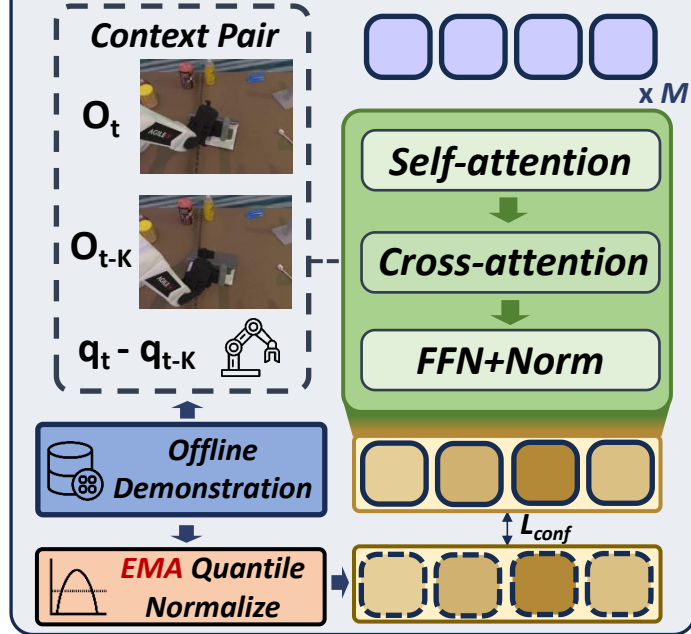
(b) VLA-Rolling Training
