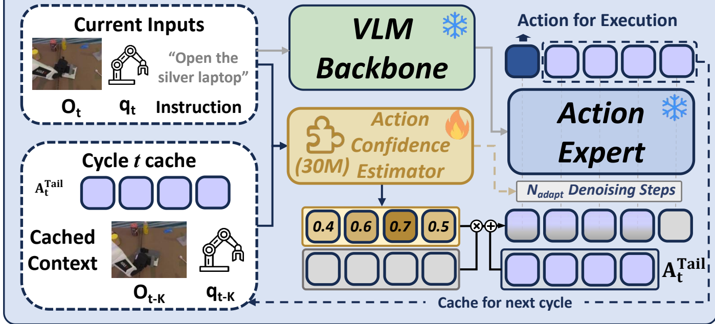
(a) Action Reuse VLA Inference Guided by VLA-Rolling
